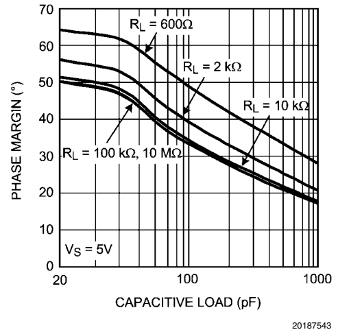
Phase Margin vs. Capacitive Load
