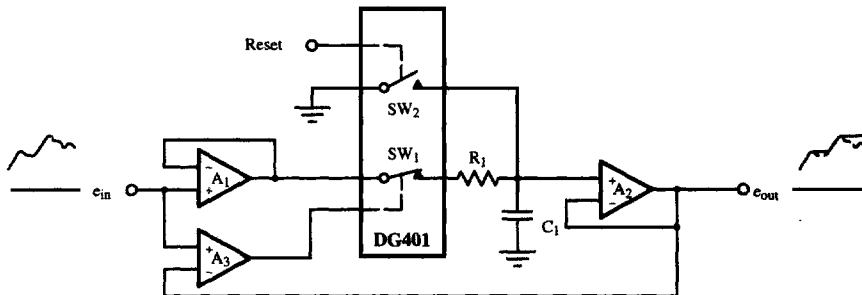
Figure 12. Positive Peak Detector
