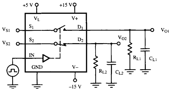
Figure 3. Break-Before-Make
