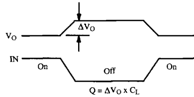
Figure 4. Charge Injection
