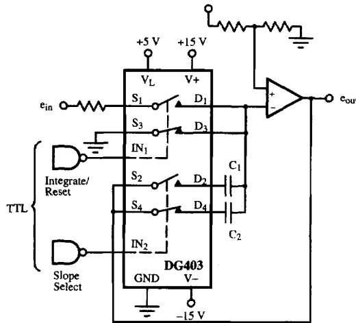
Figure 10. Dual Slope Integrator
