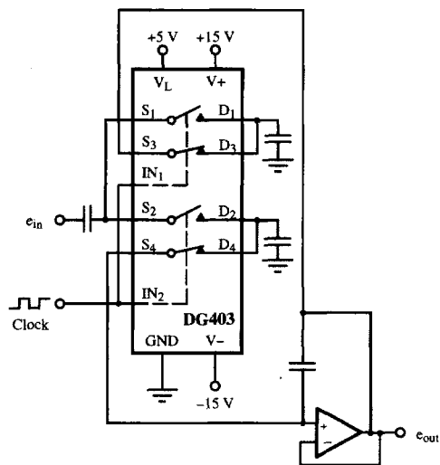
Figure 11. Band-Pass Switched Capacitor Filter
