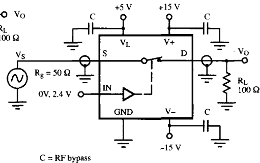
Figure 6. Insertion Loss
