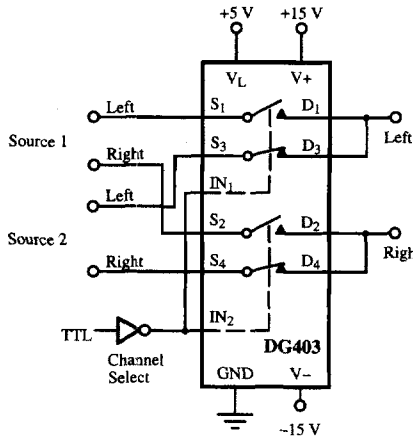
Figure 9. Stereo Source Selector
