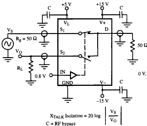
Figure 7. Crosstalk
