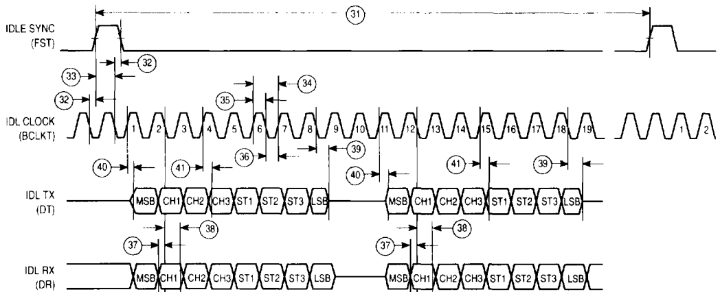
Figure 5. IDL Interface Timing
