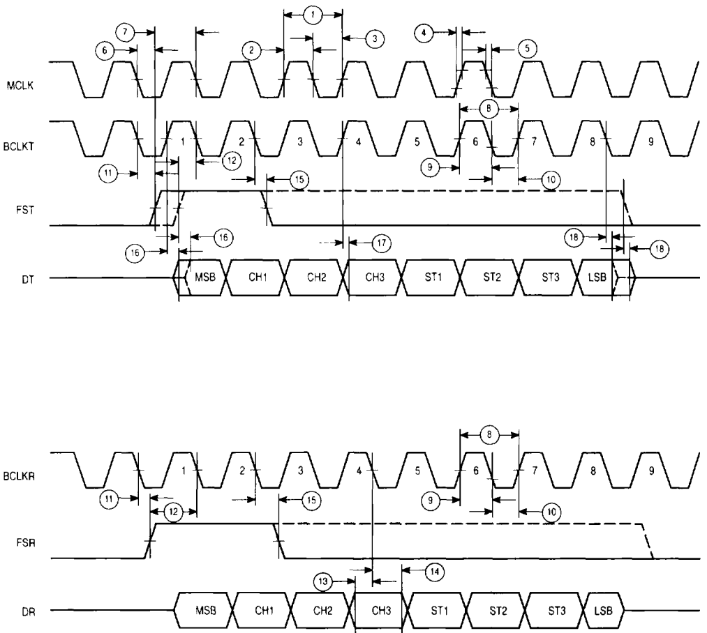
Figure 3. Long Frame Sync Timing
