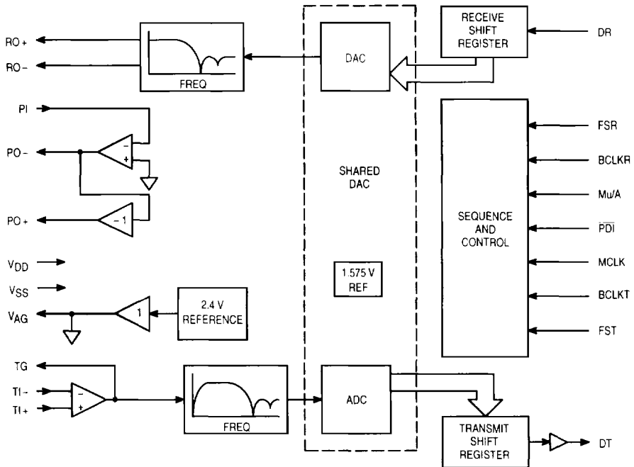
Figure 1. MC145480 PCM Codec-Filter Block Diagram
