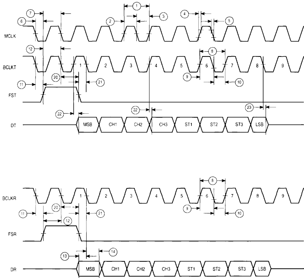
Figure 4. Short Frame Sync Timing
